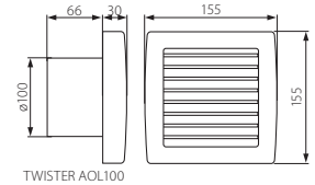
TWISTER AOL100
