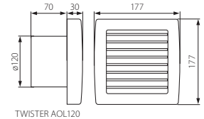
TWISTER AOL120
