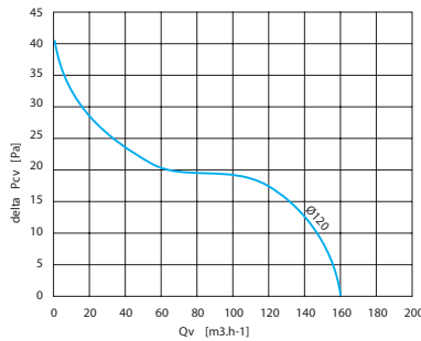
TWISTER AOL120
