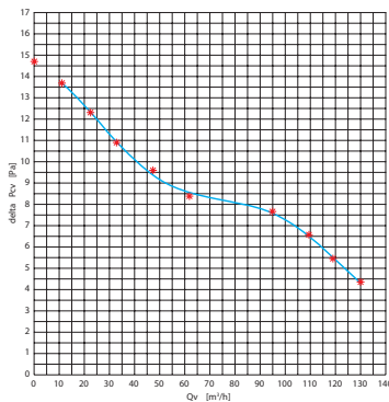
TWISTER AOL100
